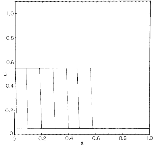
FIG. 6. A one-dimensional problem. The initial distribution is u(x, 0) = 0.05 for x > 0 , and u(0, t) = 0.55 . The solution u(x, t) at every k_2 = 7 time steps is plotted. The wave is a pure shock for all t \geq 0 .
