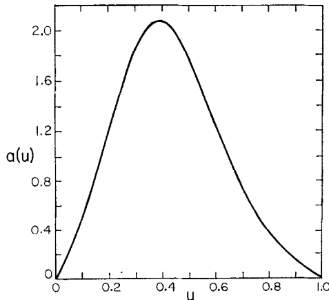
FIG. 9. The function a(u) in (10).
