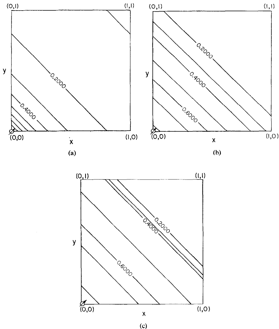
FIG. 8. A two-dimensional problem. (a) Contours of u(x, y; t) for t = 0 (initial distribution). (b) Contours of u(x, y; t) after k_2 = 7 time steps. (c) Contours of u(x, y; t) after 2k_2 = 14 time steps.
